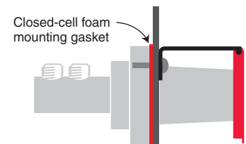
THROUGH-MOUNT PANEL .070-.090" CAT. NO. CL40WTC-L-.187
