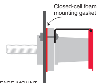
SURFACE-MOUNT CAT. NO. CL40WTC-L-.125
