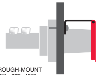
THROUGH-MOUNT PANEL .070-.090" CAT. NO. CL40WTC-L-.187
