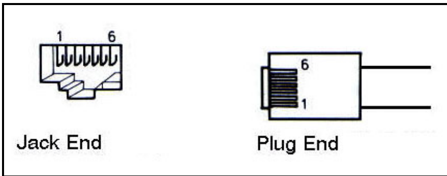
Figure 1 - RJ14/ RJ25 Positions
