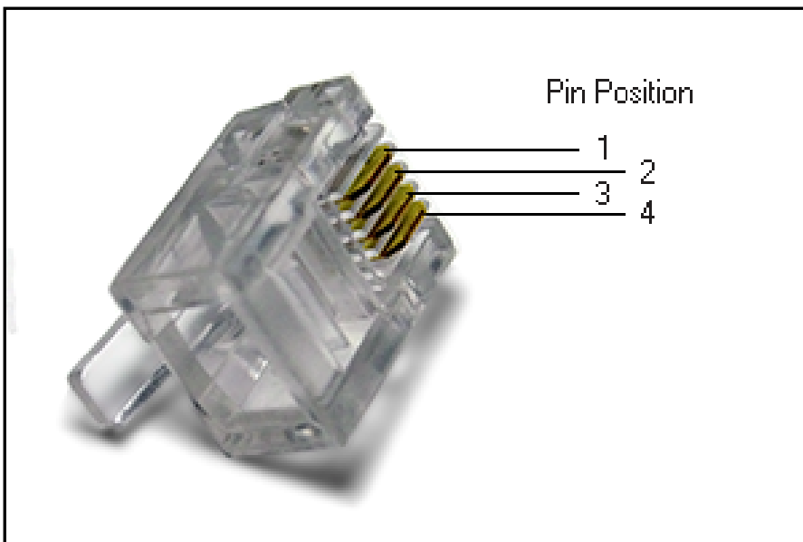
Figure 2 - RJ14 (6P4C) Conductor Pin Positions
