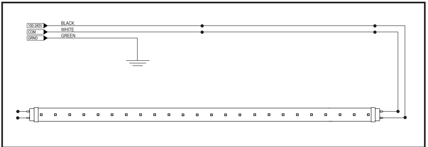
Wiring Diagram 1
