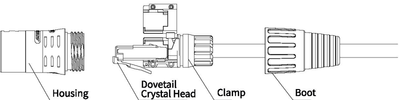
● SE8MC-02-30-LOD(Parts Diagram)
