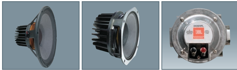
2255H 15" DIFFERENTIAL DRIVE® LOUDSPEAKER
